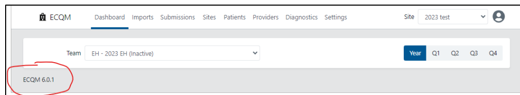
Figure 6-6: ECQM Version
