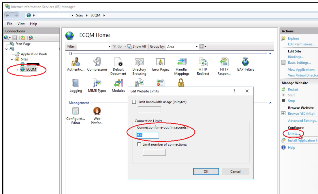
Figure 5-28: Connection time-out
