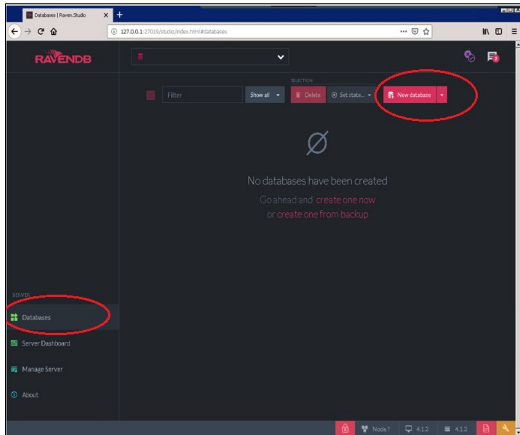
Figure 5-13: Database selection
