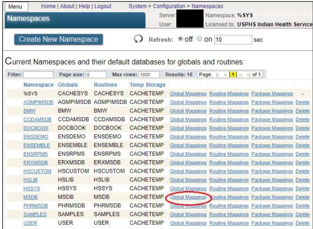
Figure 4-21: Namespaces window with Global Mappings
