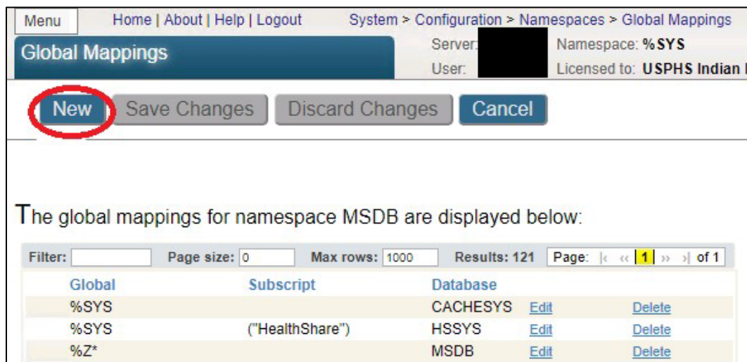
Figure 4-22: Global Mappings window
