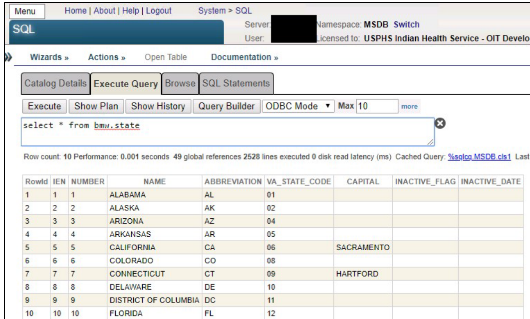
Figure 4-20: Example of test query
