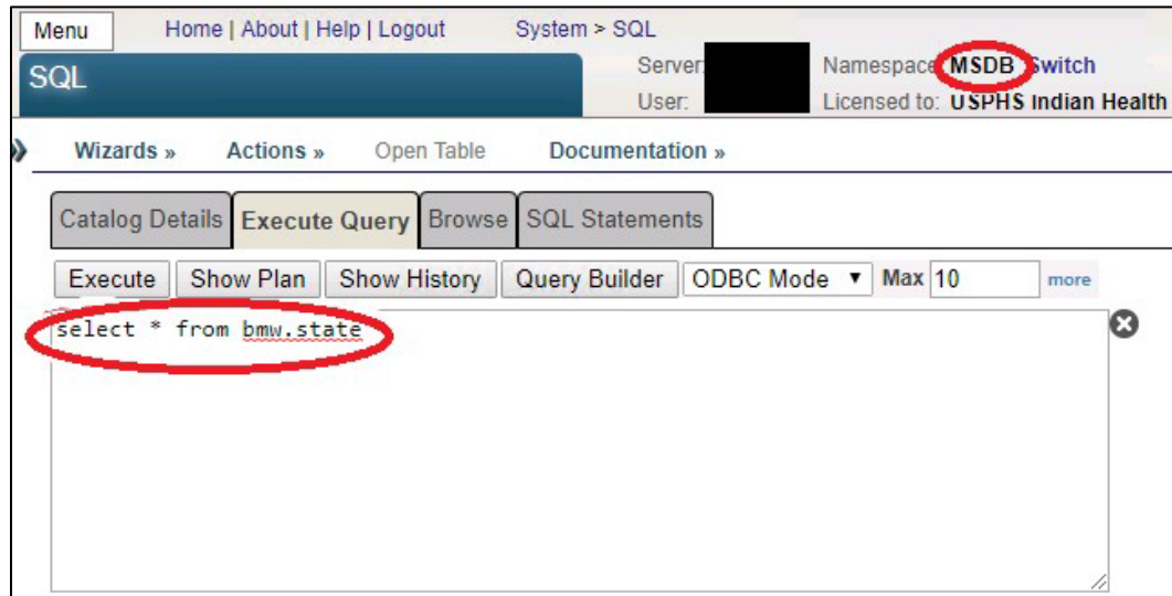
Figure 4-19: Execute SQL Query window
