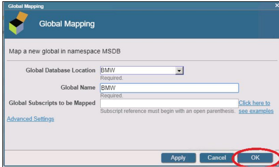
Figure 4-23: Global Mapping dialog
