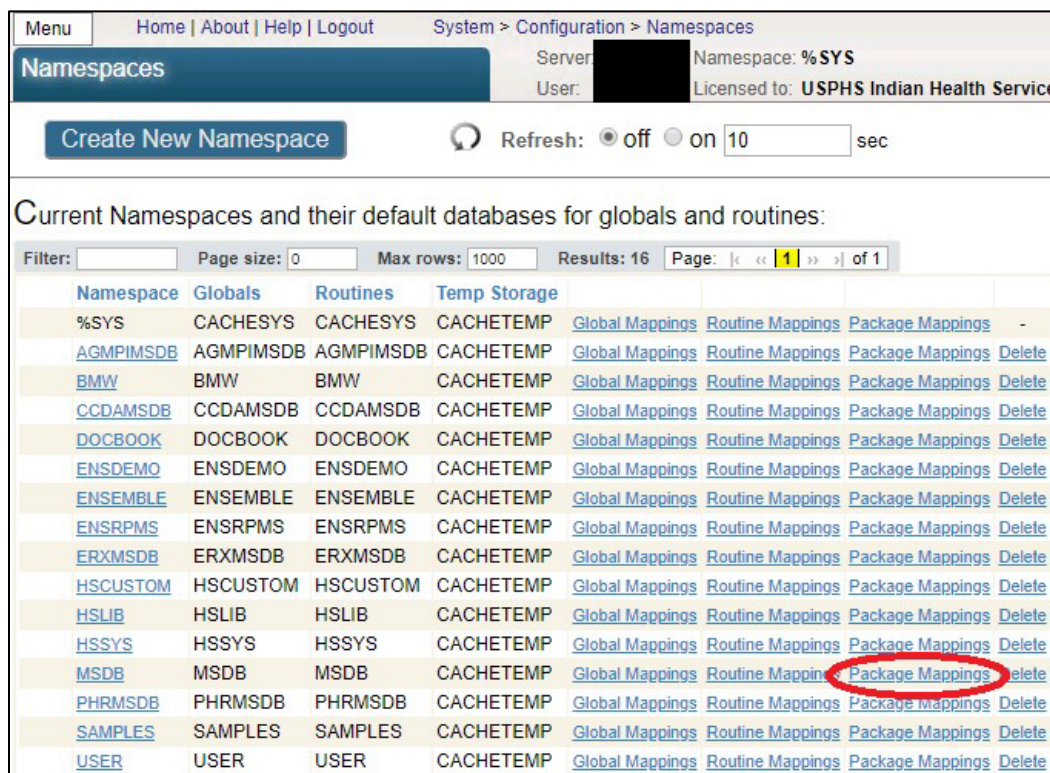
Figure 4-15: Namespaces window with Package Mappings
