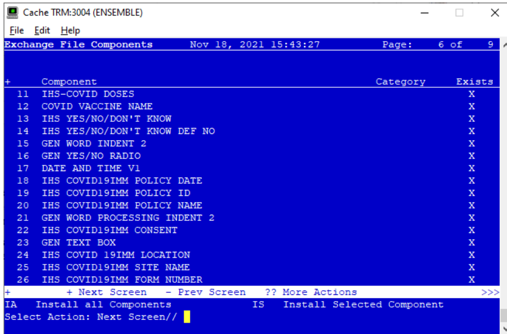
Figure 5-4: Exchange entry
