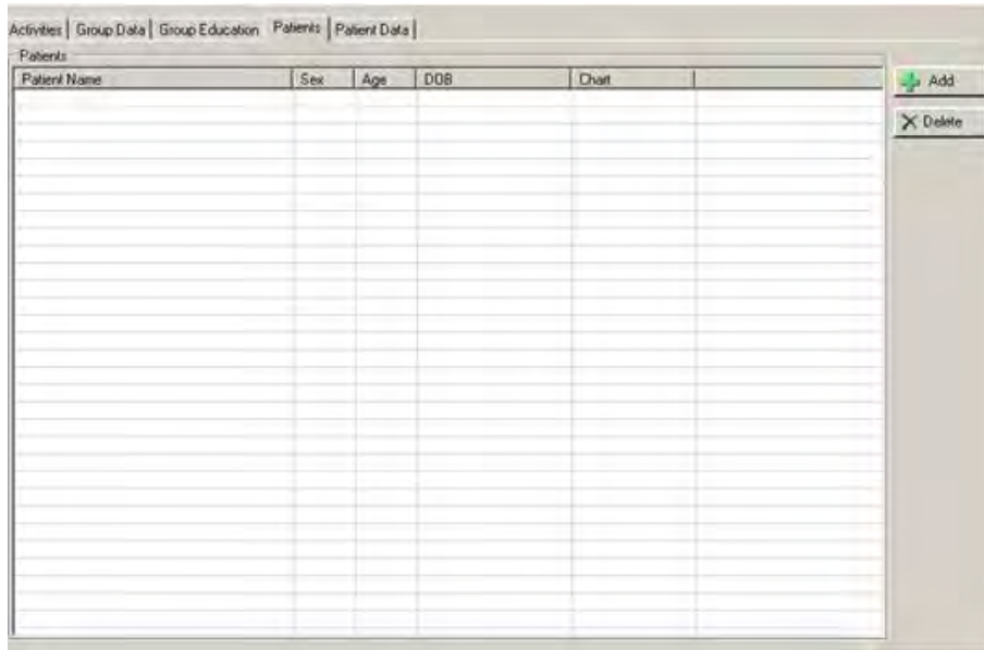
Figure 5-46: Patients tab
