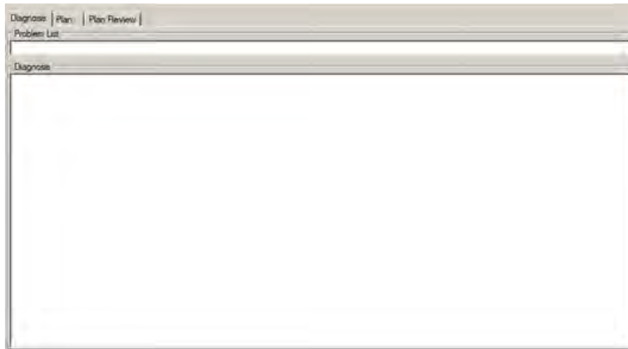
Figure 10-25: Diagnosis tab
