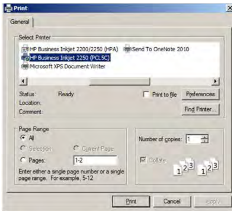
Figure 2-14: Print dialog
