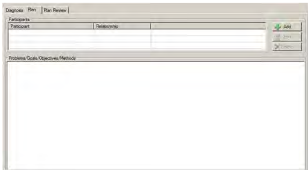
Figure 10-26: Plan tab
