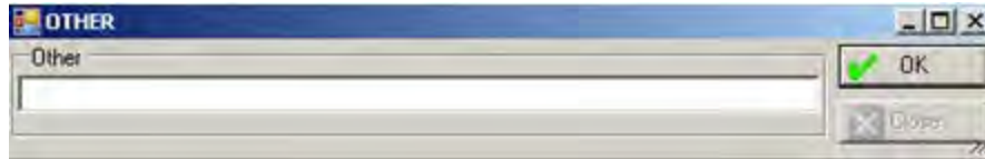
Figure 11-29: Other dialog
